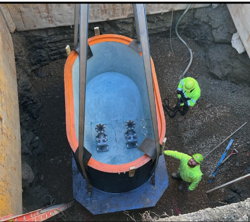
Pumped-Out Wetwell/Valve Vault Excavation
